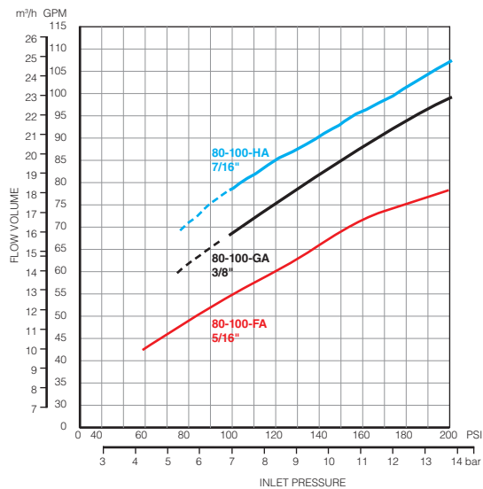
Flow Versus Pressure for Dual-Nozzle TANK MAN
