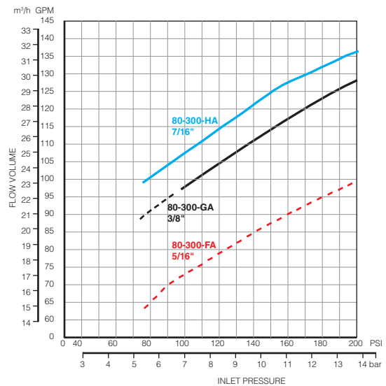
Flow Versus Pressure for Triple-Nozzle TANK MAN
